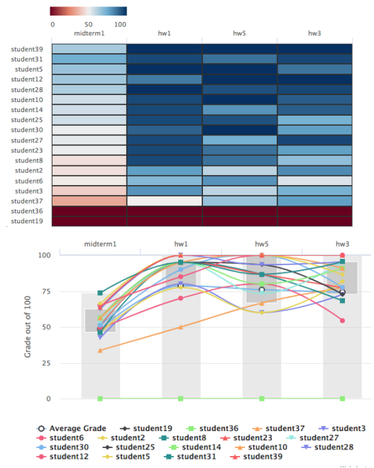
Figure 5: The flood of data contained in a grade book can be made sense of by using analytics such bi-clustering algorithms. Here one bi-cluster extracted by the CPB algorithm is shown spanning 18 students and 4 grades. This bi-cluster highlights that the grades on three homeworks and one midterm are correlated.
