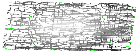
Figure 3: Map of Minneapolis, MN colored by distances to the center of the map.
