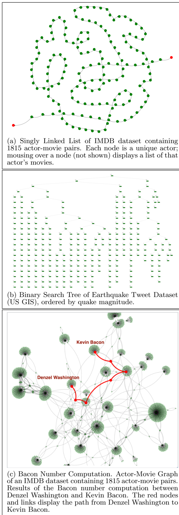
Figure 4: BRIDGES Project Examples
