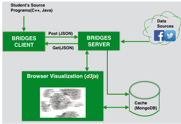
Figure 1: BRIDGES System. Based on a client-server architecture; a user constructs data structure programs using the BRIDGES client classes (Fig. 3) in Java or C++. The data structure representation is sent to the server by the client as a JSON string. After parsing and user authentication, the server stores the assignment on the MongoDB and displays the data structure on a specific web link using D3. The server also has interfaces to retrieve data from external sources upon user requests for use in their programs.
